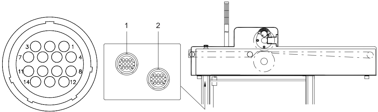
Figura 25 Interfaces SMEMA
